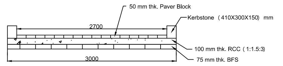
Cross Section of "A-A" Path Way
